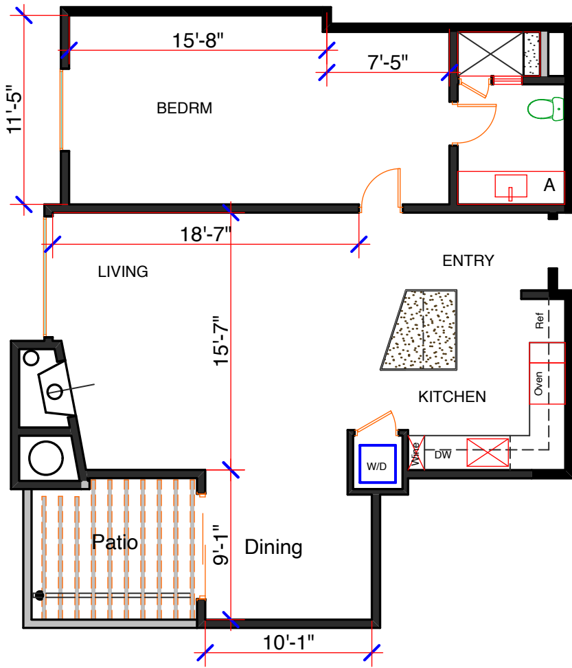
Plan PH5 Unit Type F
